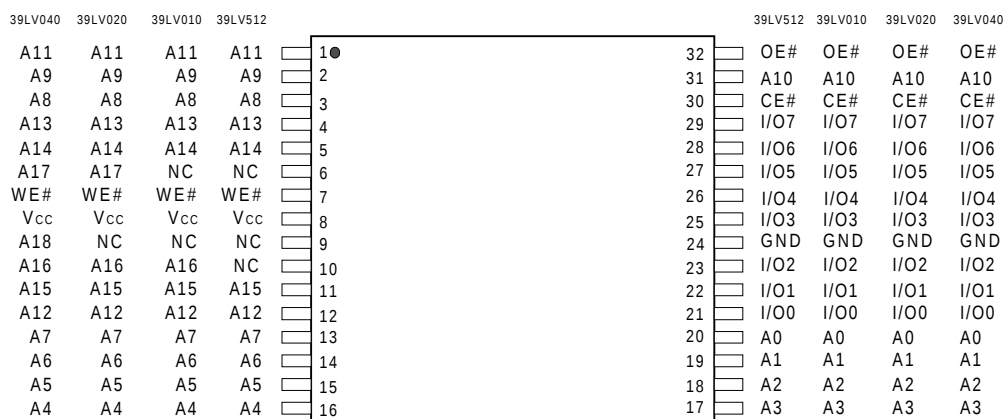
32-Pin VSOP
