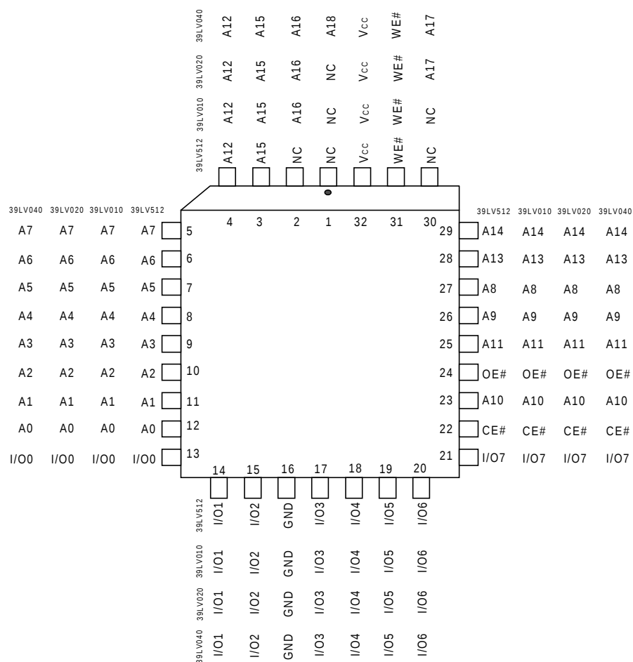
32-Pin PLCC
